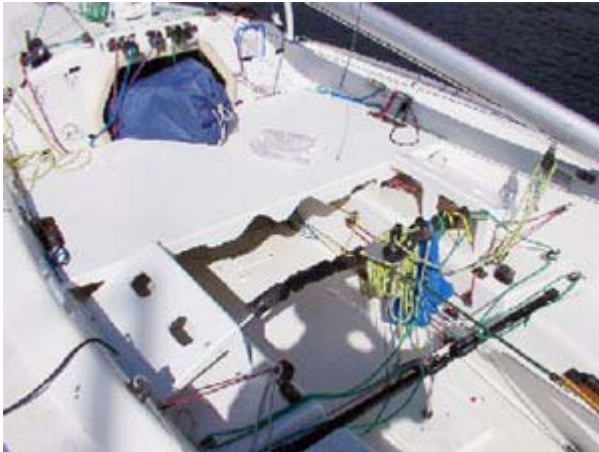
CAN – Transfer seat, bench for main trimmer and raised mainsheet block
